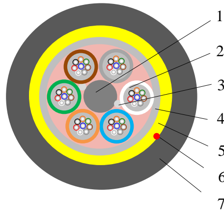
Cable Section Sketch Map
